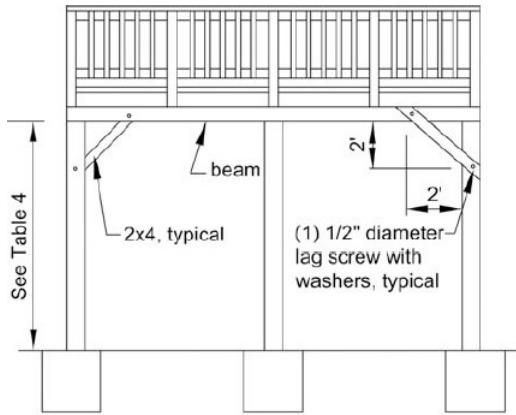
DIAGONAL BRACING PARALLEL TO BEAM
